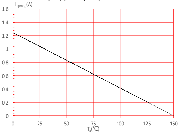
FIG.5: On-state characteristics
